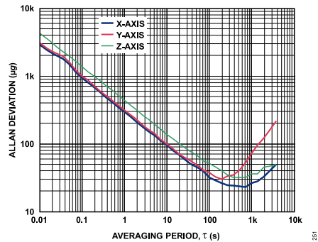
Figure 52. Root Allan Deviation
