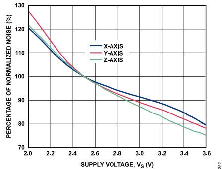
Figure 53. Normalized Noise vs. Supply Voltage, V_S
