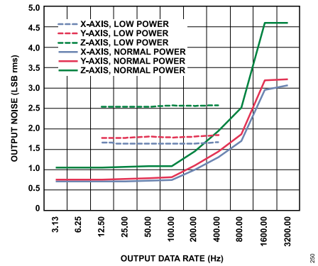
Figure 51. Noise vs. Output Data Rate for Normal and Low Power Modes, Full-Resolution (256 LSB/g)
