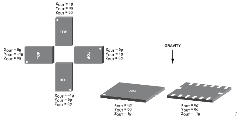
Figure 58. Output Response vs. Orientation to Gravity
