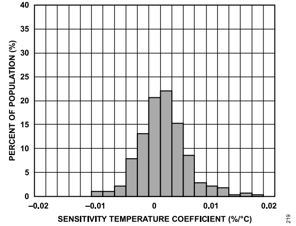
Figure 19. X-Axis Sensitivity Temperature Coefficient, V_S = 2.5 V
