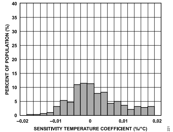
Figure 21. Z-Axis Sensitivity Temperature Coefficient, V_S = 2.5 V
