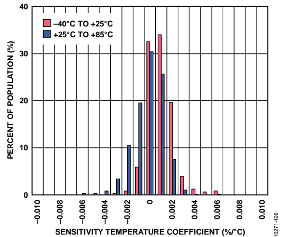
Figure 27. Z-Axis Sensitivity Temperature Coefficient, V_s = 2.5\text{ V}
