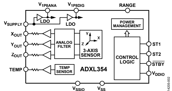
Figure 1. ADXL354
