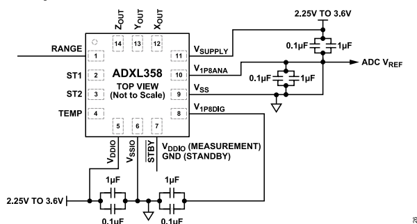
Figure 26. ADXL358 Application Circuit
