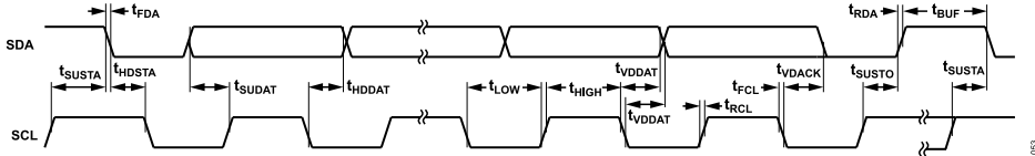
Figure 17. I 2 C Interface Timing Diagram
