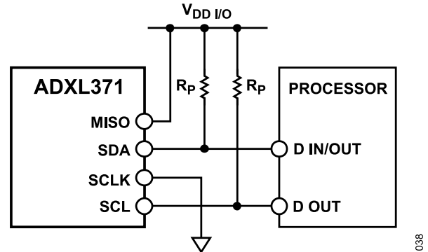
Figure 49. I 2 C Connection Diagram (ADXL371 Device ID = 0x53)
