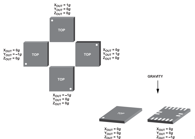
Figure 56. Output Response vs. Orientation to Gravity
