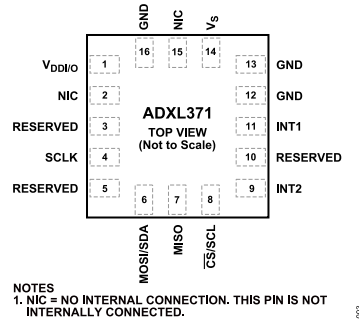
Figure 12. Pin Configuration (Top View)
