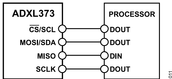
Figure 50. 4-Wire SPI Connection Diagram
