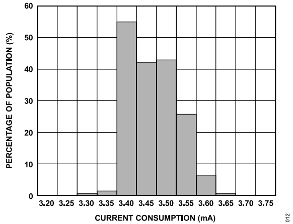
Figure 11. Current Consumption at 25°C ( V_{RATIO} = 5\text{ V} )
