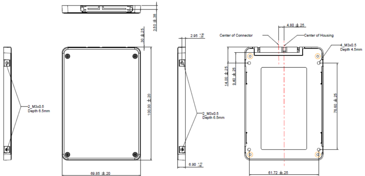
Figure 10-1 Physical Dimensions
