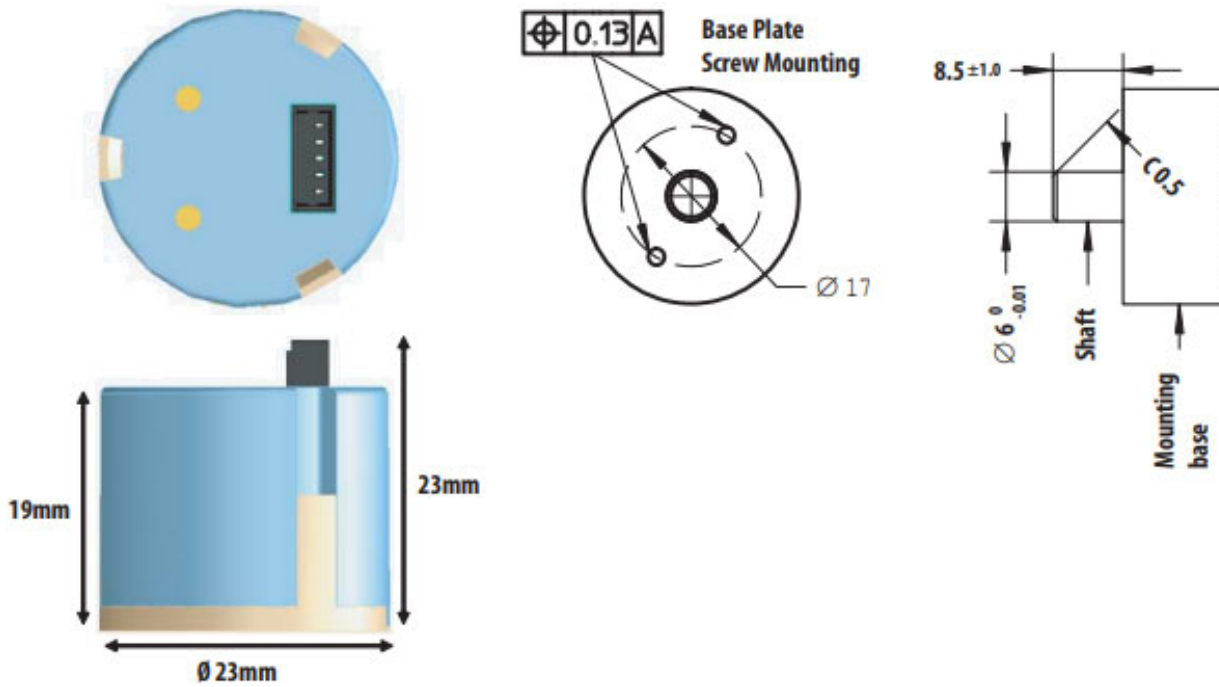
Figure 1: Package and Recommended Mounting Dimensions
