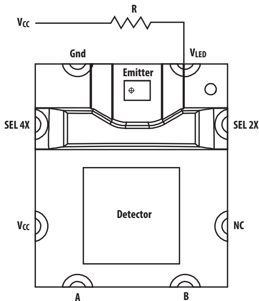
Figure 4: Resistor Placement
