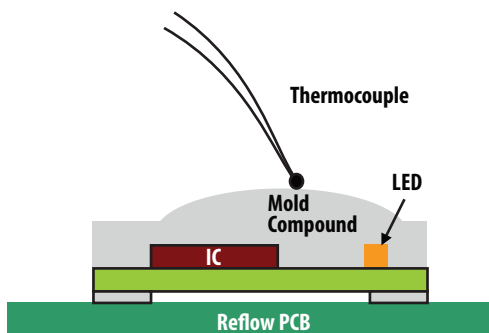
Figure 11: Thermocouple Placement
