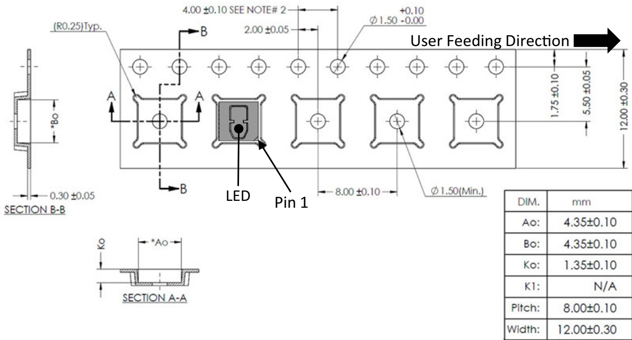
Figure 11: Tape and Reel
