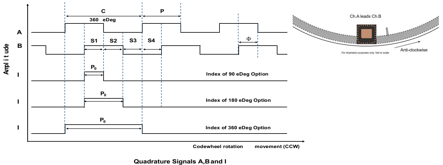
Figure 3: Sample of Output Waveforms
