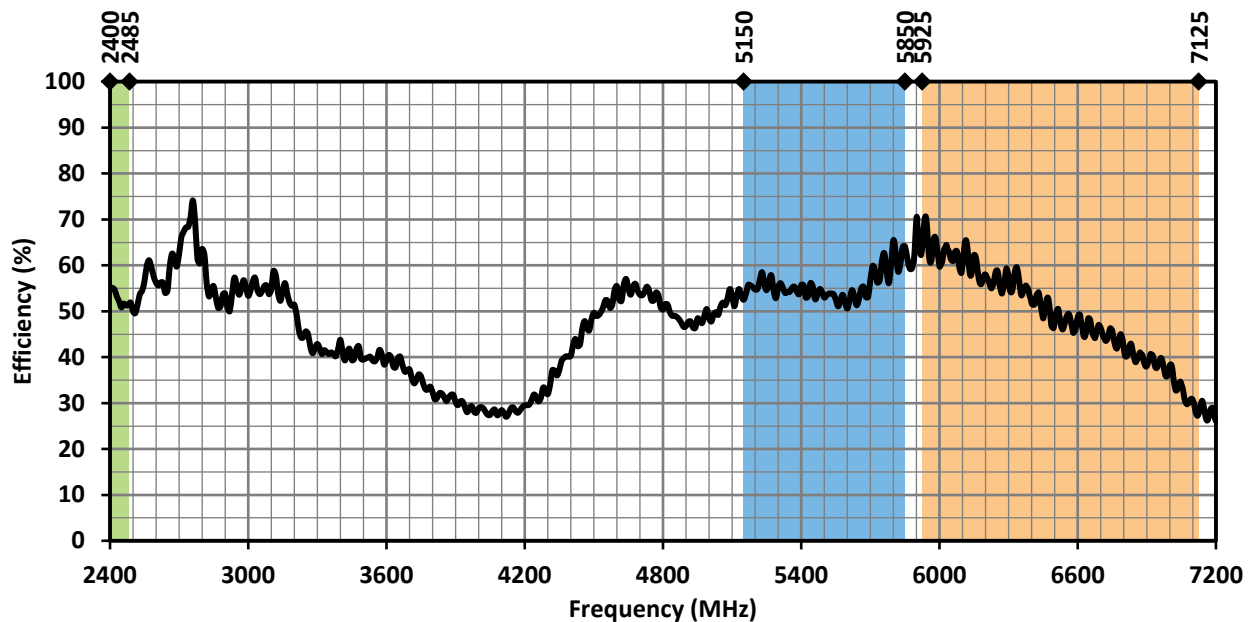
Figure 7. ANT-W63-MSA-TH1 Radiation Efficiency with Frequency Band Highlights
