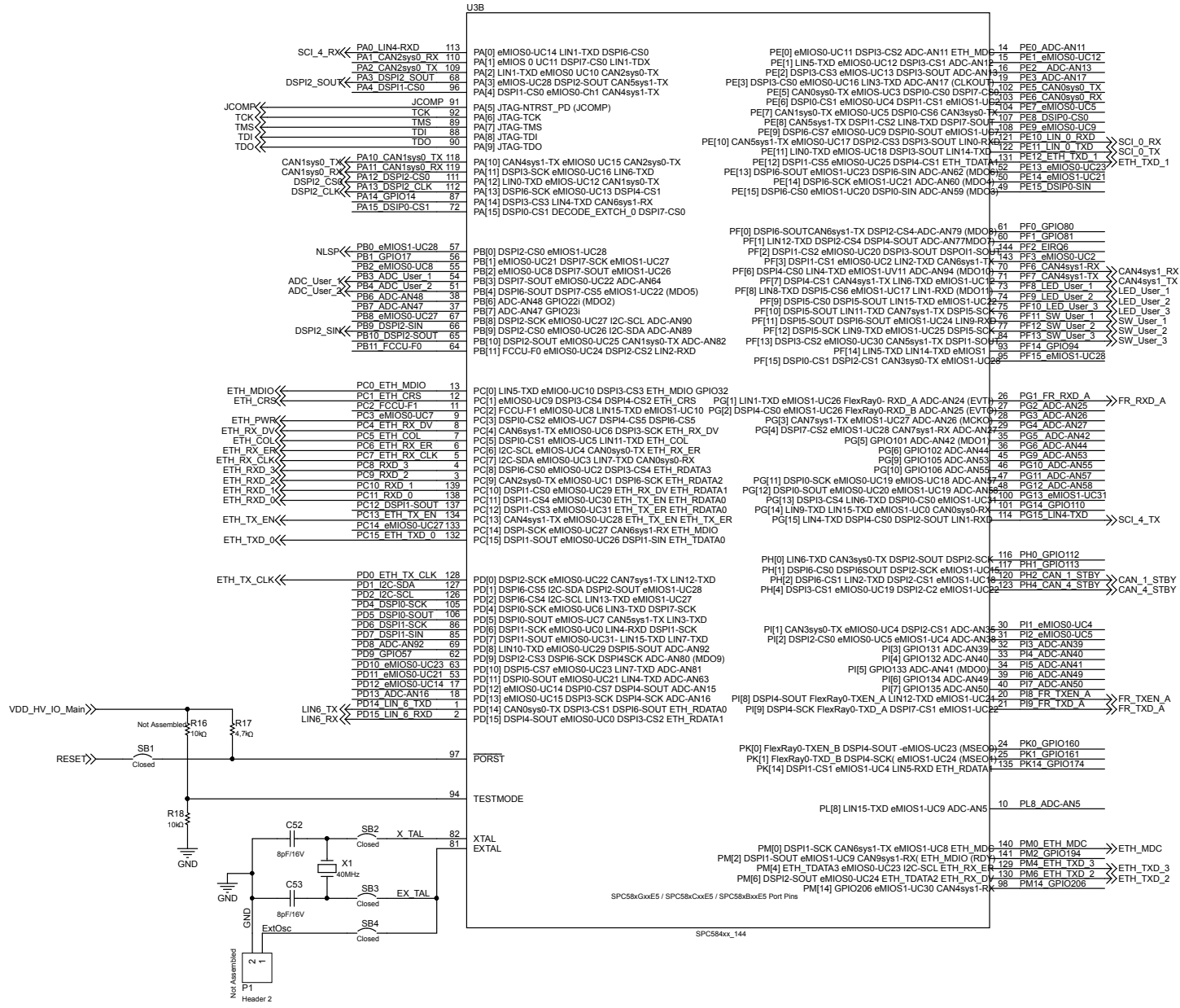
Figure 12. AEK-MCU-C4MLIT1 schematic - MCU I/O signals
