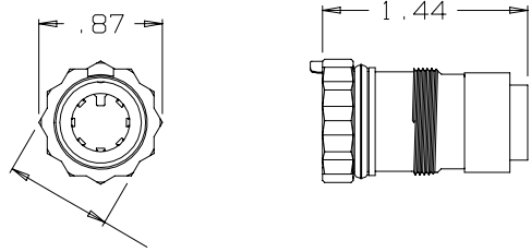
AJ-107-29 JACK BODY ASSEMBLY (1 REQ'D)
