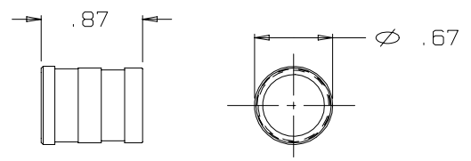
AP-107-4 SLEEVE (1 REQ'D)
