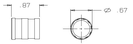
AP-107-4 SLEEVE (1 REQ'D)
