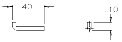
AP-107-9 RETAINER PIN SCALE 2:1 (1 REQ'D)
