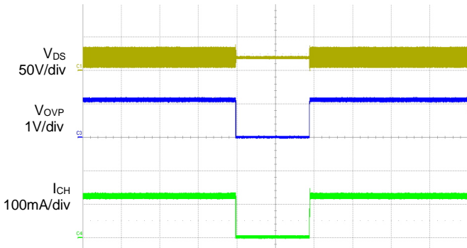
Time: 200ms/div
