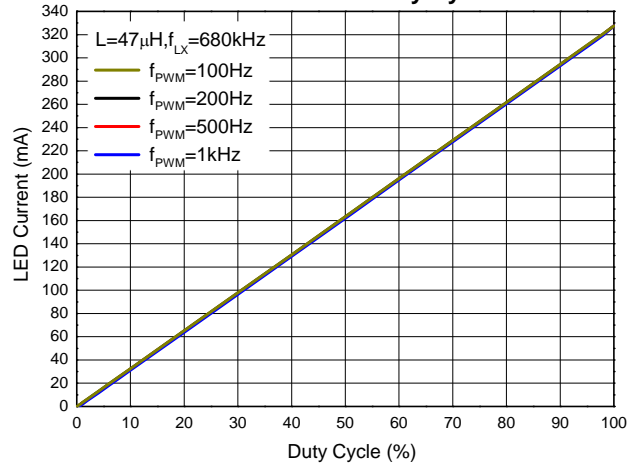
PWM Dimming ( V_{IN}=16\text{V} , 3 LEDs, L=47\mu\text{H} , R_S=0.3\Omega ) LED Current vs. Duty Cycle
