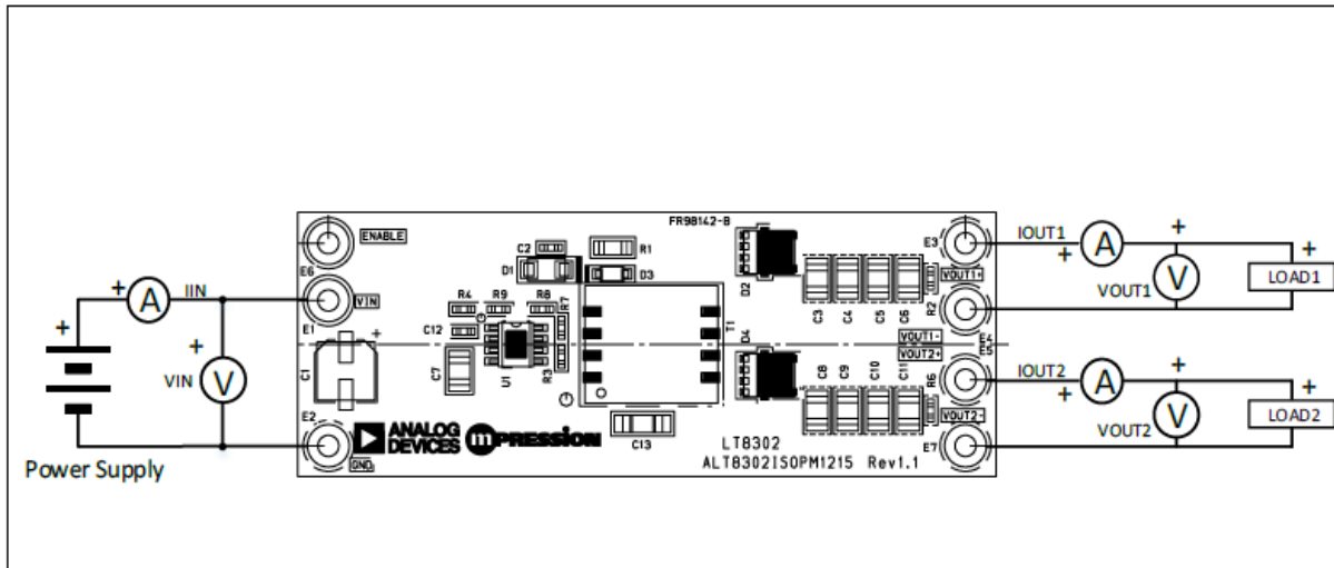
Figure 7-1 Measuring Circuit
