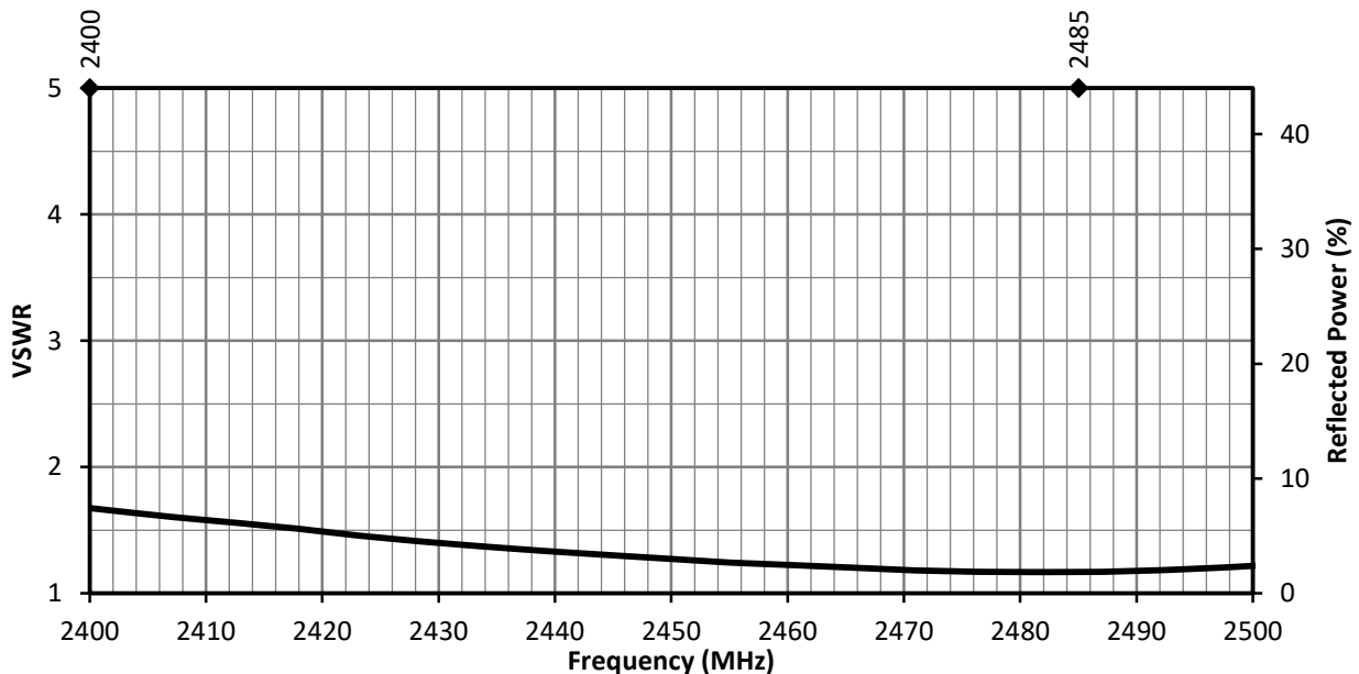
Figure 2. ANT-2.4-FPC-LV Antenna VSWR
