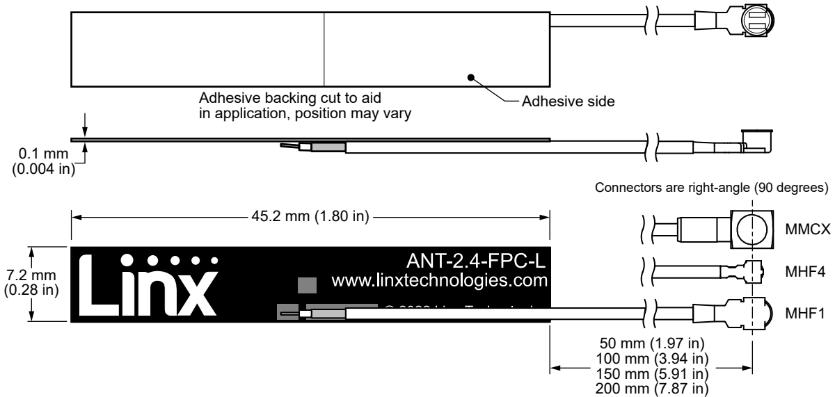
Figure 1. ANT-2.4-FPC-LV Series Antenna Dimensions
