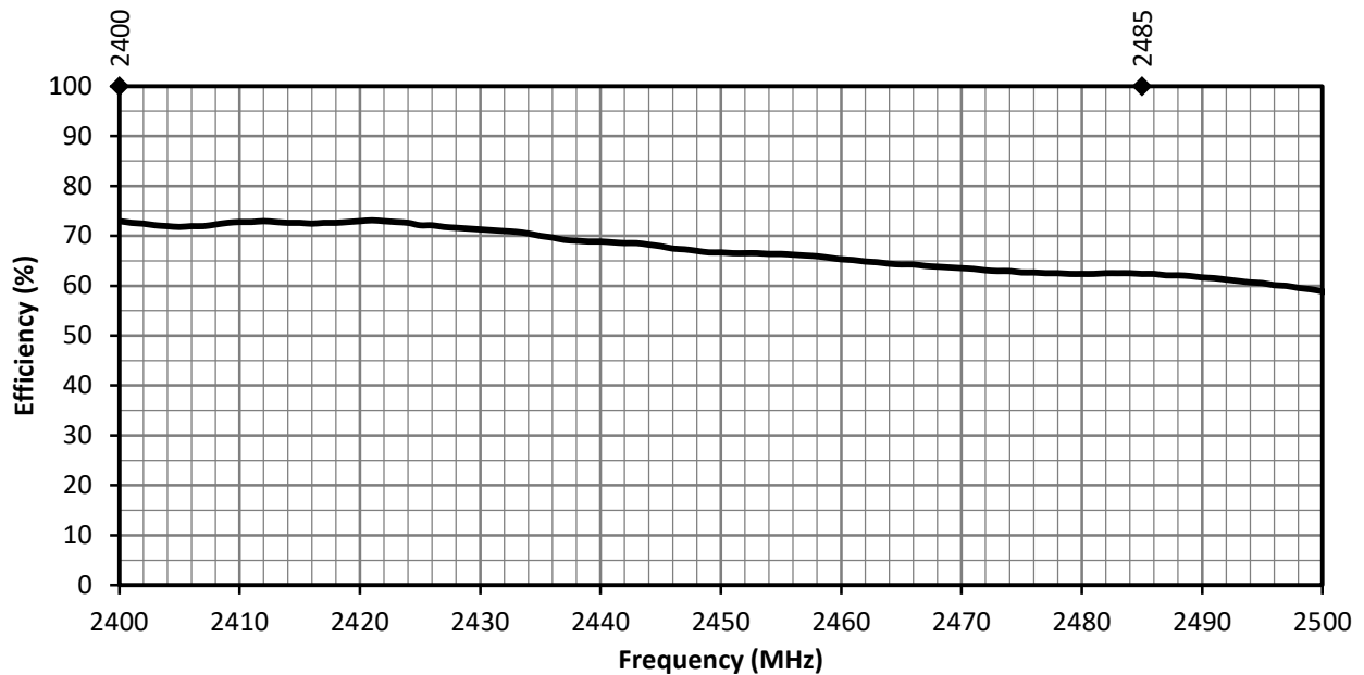
Figure 6. ANT-2.4-FPC-LV Antenna Radiation Efficiency
