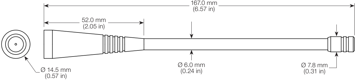
Figure 6. CW 450 MHz Antenna Dimensions
