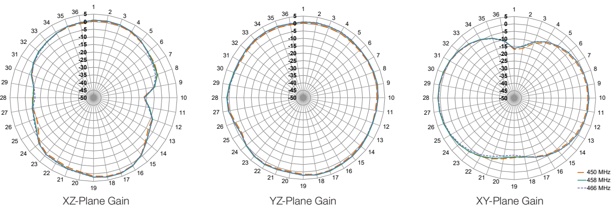
Figure8. Radiation Patterns for CW 450 MHz Antenna
