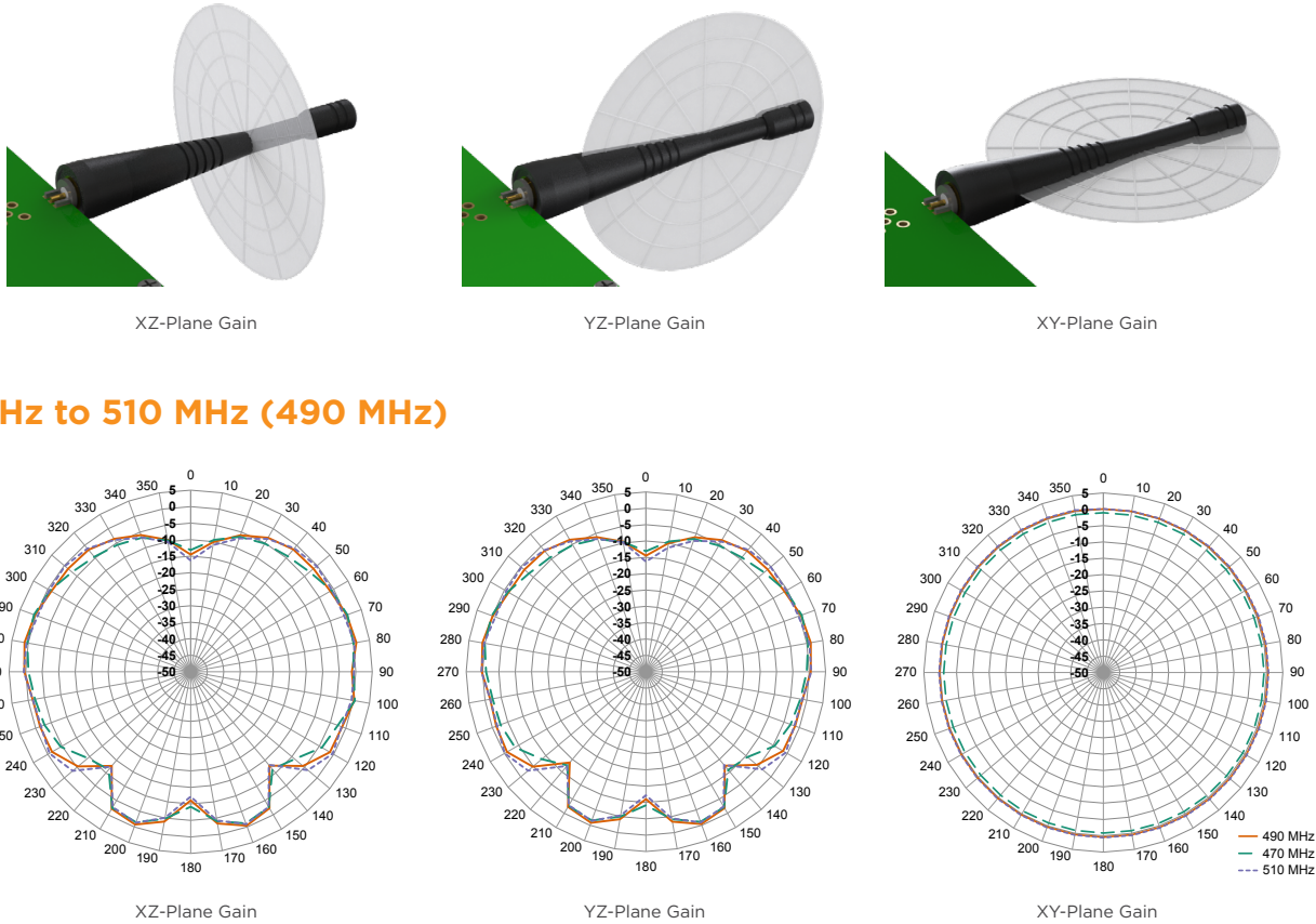
Figure 8. Radiation Patterns for CW 490 MHz Antenna
