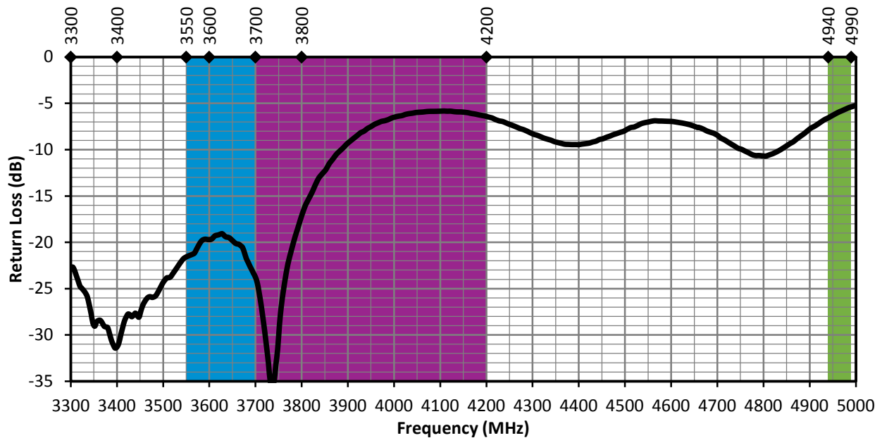
Figure 12. ANT-5GMWS1-SMA Return Loss, Edge-Bent
