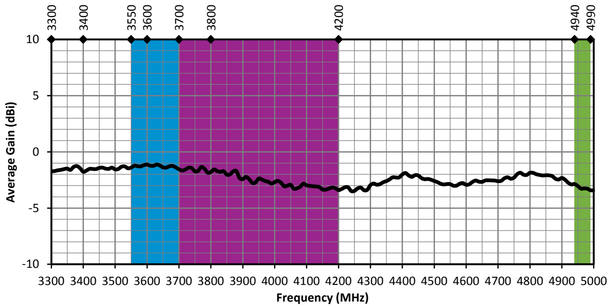
Figure 7. AANT-5GMW-SMA Series Antenna Average Gain, Straight
