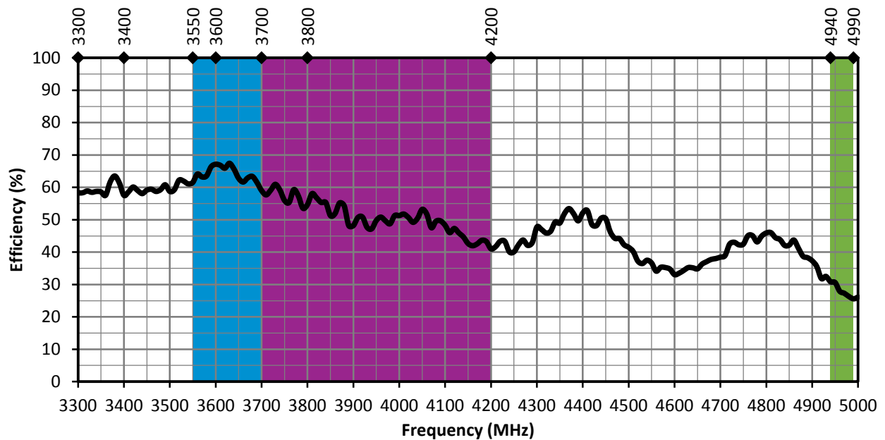
Figure 15. ANT-5GMWS1-SMA Antenna Efficiency, Edge-Bent
