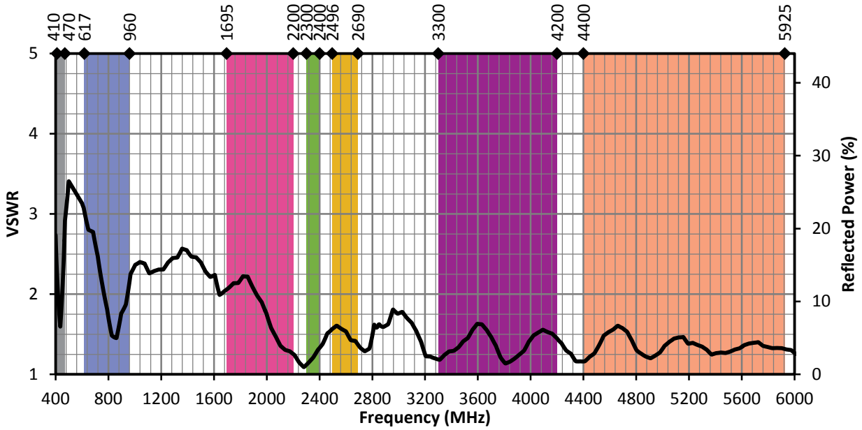
Figure 2. ANT-5GW-SPS1 VSWR
