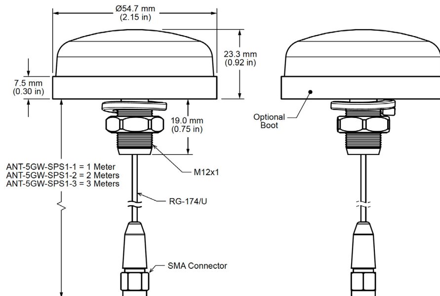
Figure 1. ANT-5GW-SPS1 Series Dimensions
