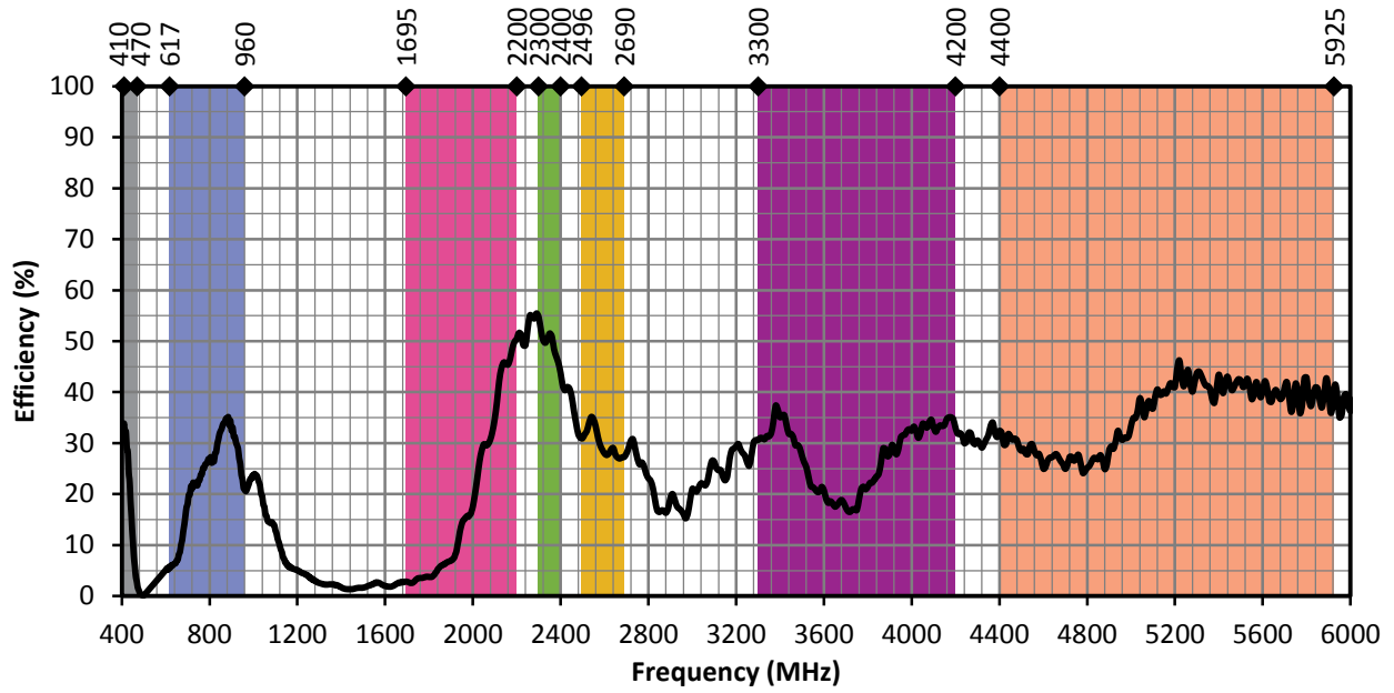
Figure 6. ANT-5GW-SPS1 Antenna Efficiency
