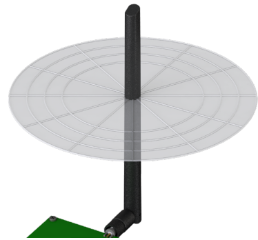
XY-Plane Gain
