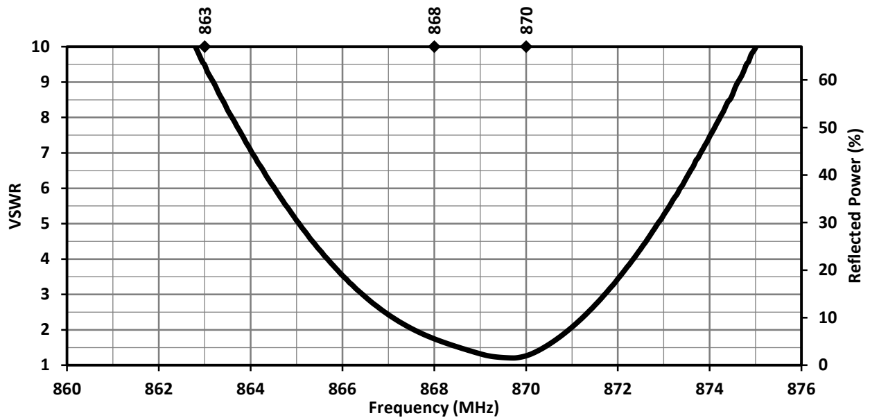
Figure 2. 868-CPA VSWR
