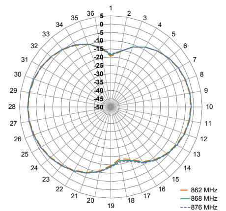
XY-Plane Gain
