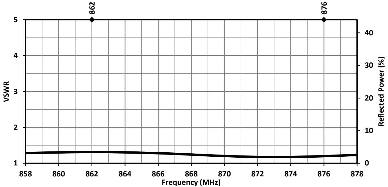
Figure 2. 868-CPA VSWR
