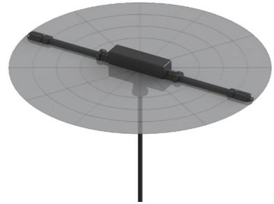
XY-Plane Gain
