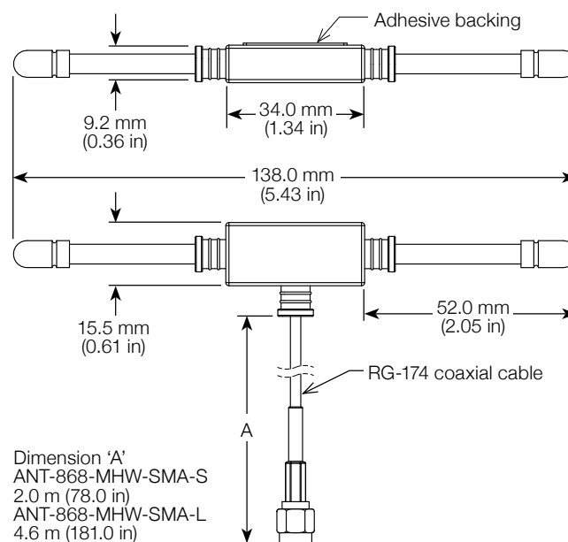
Figure 1. ANT-868-MHW Dimensions
