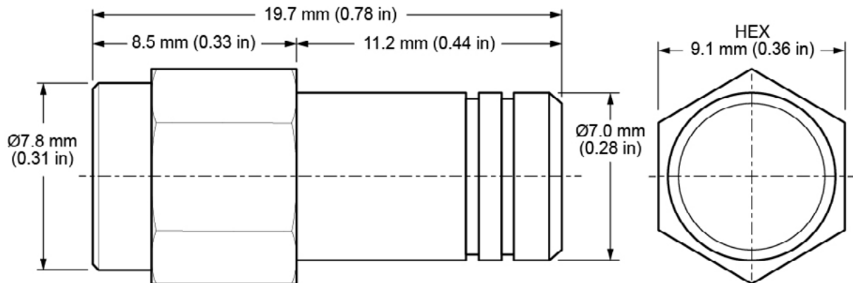
Figure 1. ANT-868-NUB-ccc Antenna Dimensions
