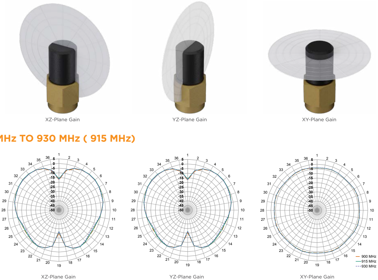
Figure 16. Radiation Patterns for ANT-915-NUB-ccc Antenna in Free Space
