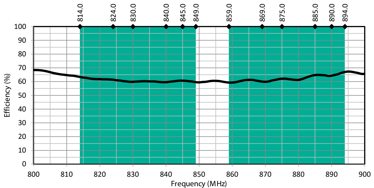
Figure 5: PW LTE Band 5 Antenna Radiation Efficiency with Band 5 Uplink/Downlink Highlights
