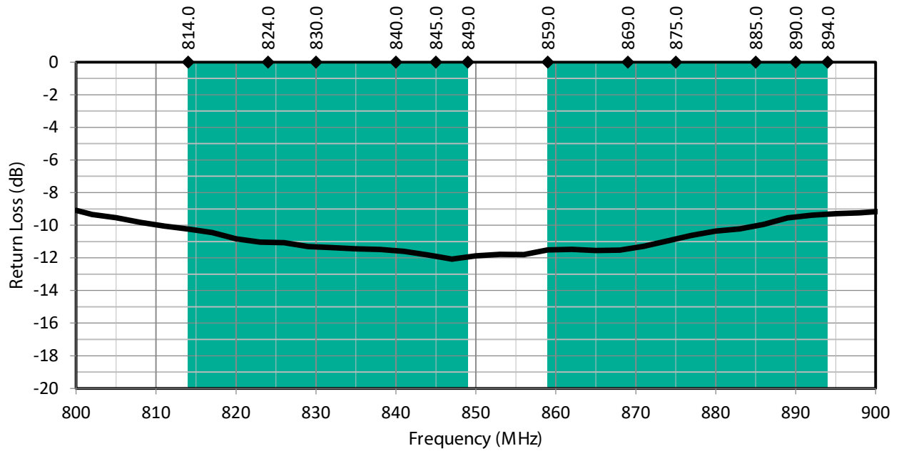
Figure 2: PW LTE Band 5 Antenna Return Loss with Band 5 Uplink/Downlink Highlights
