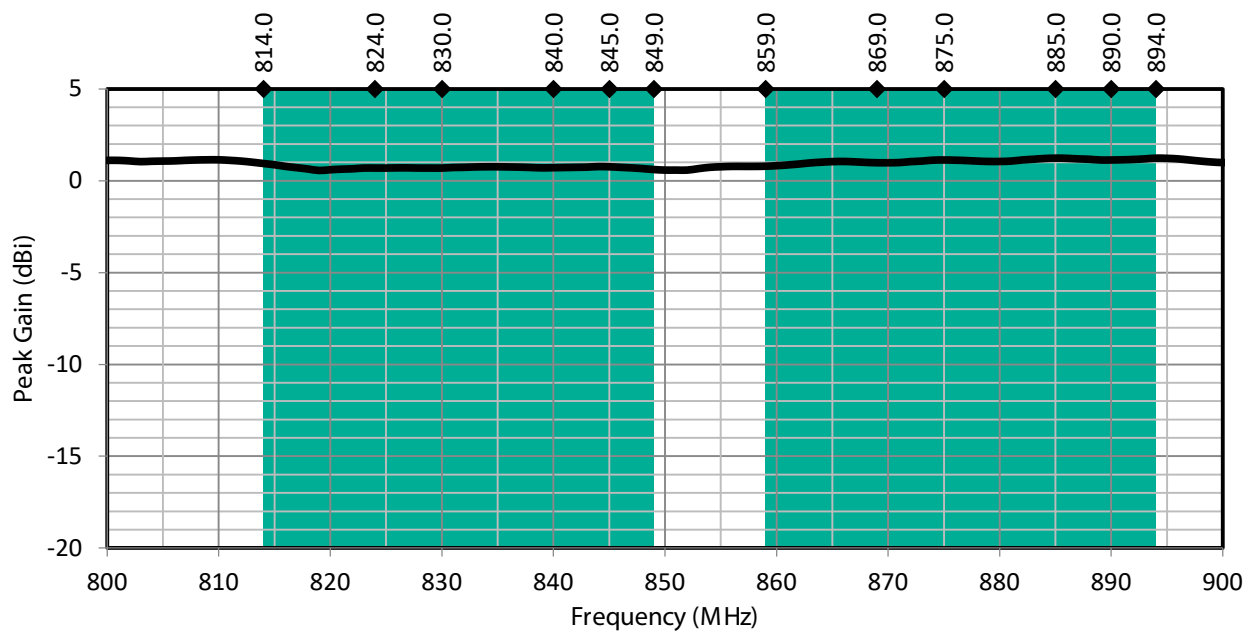
Figure 3: PW LTE Band 5 Antenna Peak Gain with Band 5 Uplink/Downlink Highlights
