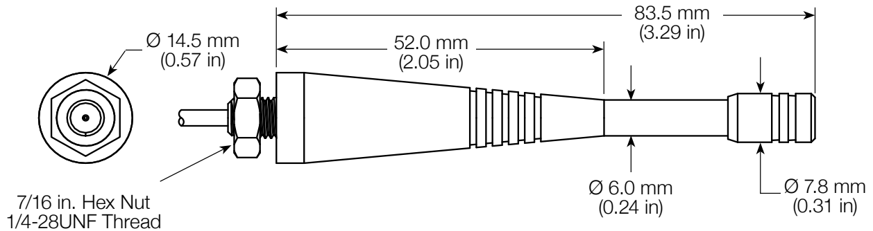
Figure 6: PW LTE Band 5 Antenna Dimensions
