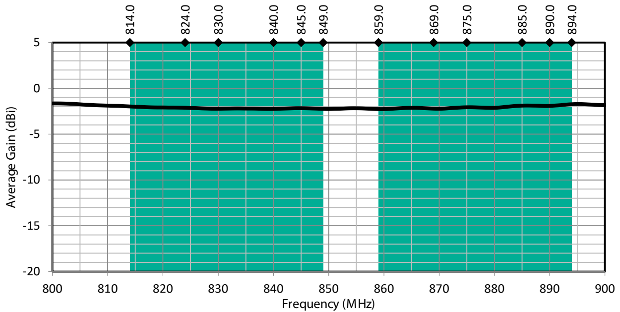
Figure 4: PW LTE Band 5 Antenna Average Gain with Band 5 Uplink/Downlink Highlights
