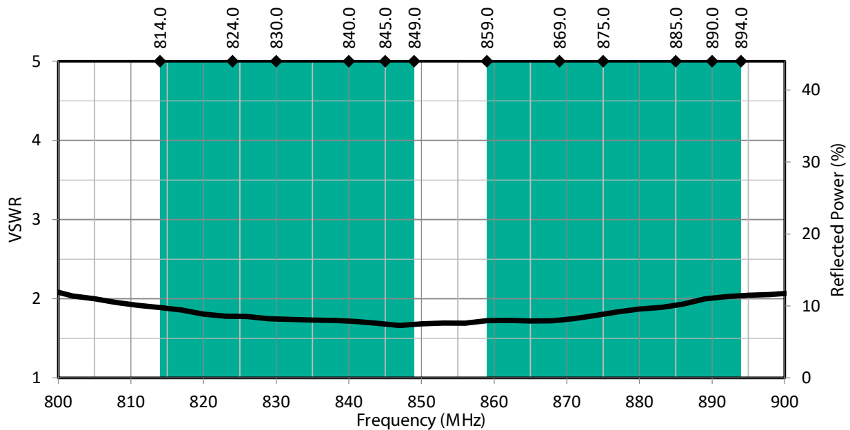
Figure 1: PW LTE Band 5 Antenna VSWR with Band 5 Uplink/Downlink Highlights
