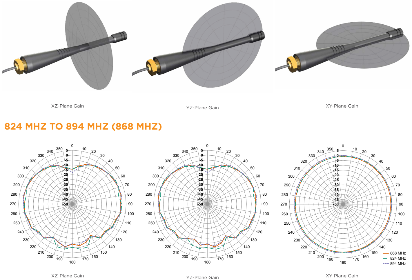
Figure 8: Radiation Patterns for PW LTE Band 5 Antenna
