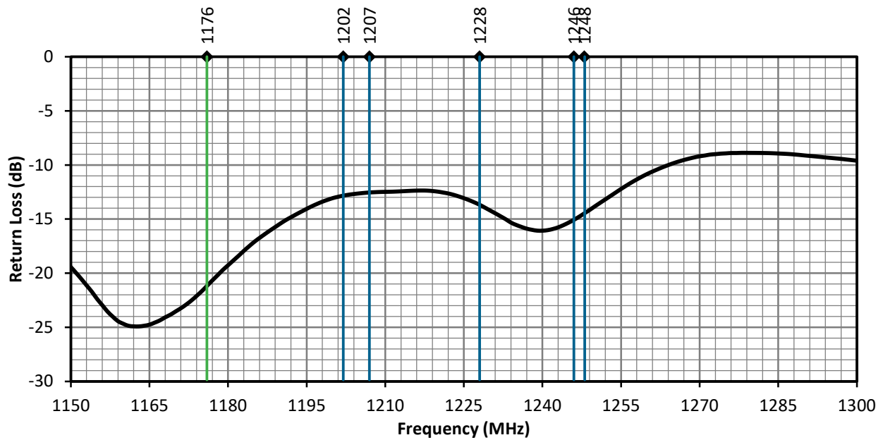
Figure 6. ANT-GCRM-L125A Return Loss, L2 and L5 Bands
