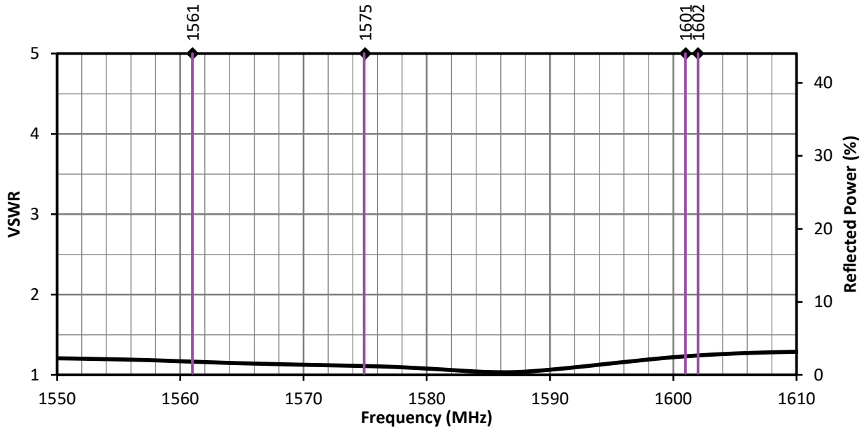
Figure 3. ANT-GCRM-L125A VSWR, L1 Band
