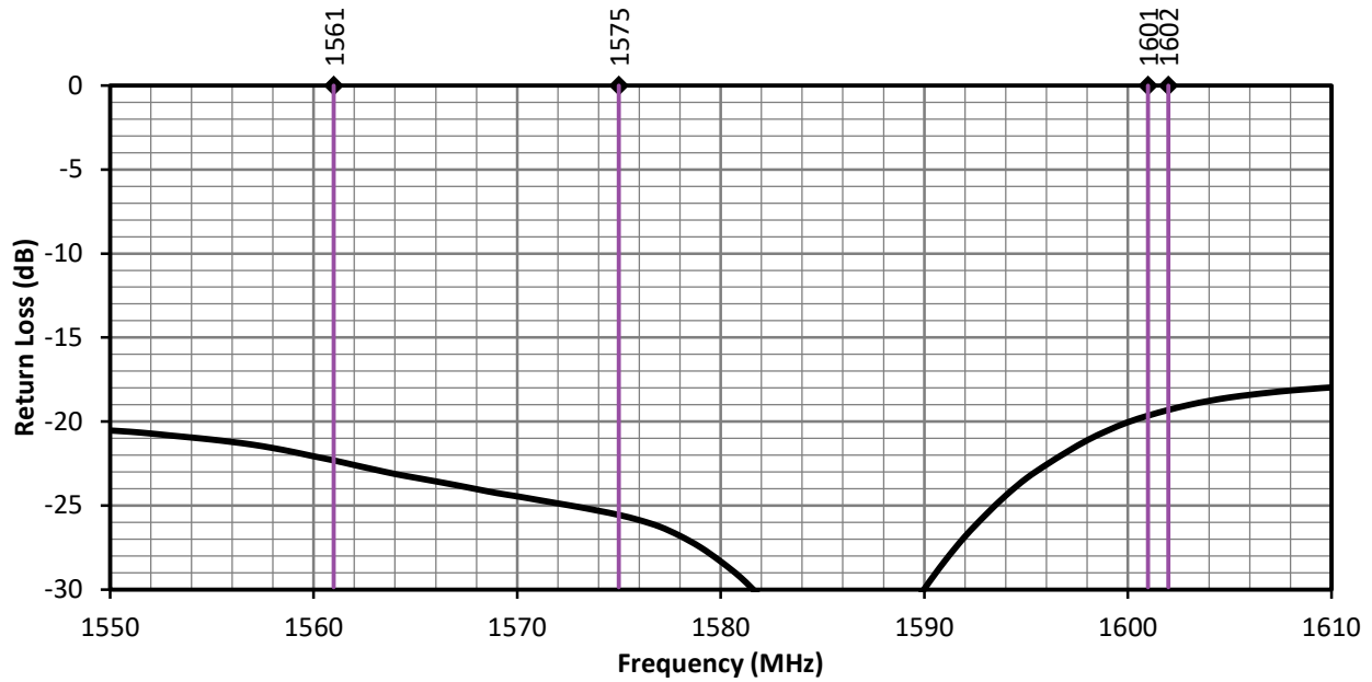
Figure 5. ANT-GCRM-L125A Return Loss, L1 Band
