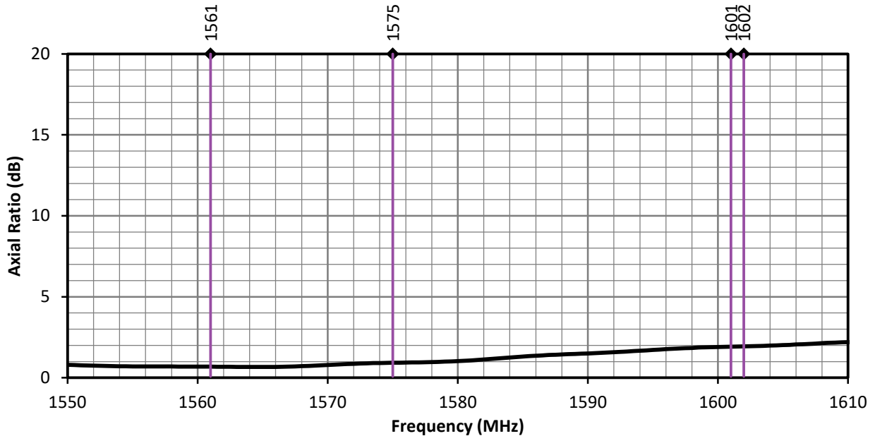
Figure 9. ANT-GCRM-L125A Antenna Axial Ratio, L1 Band
