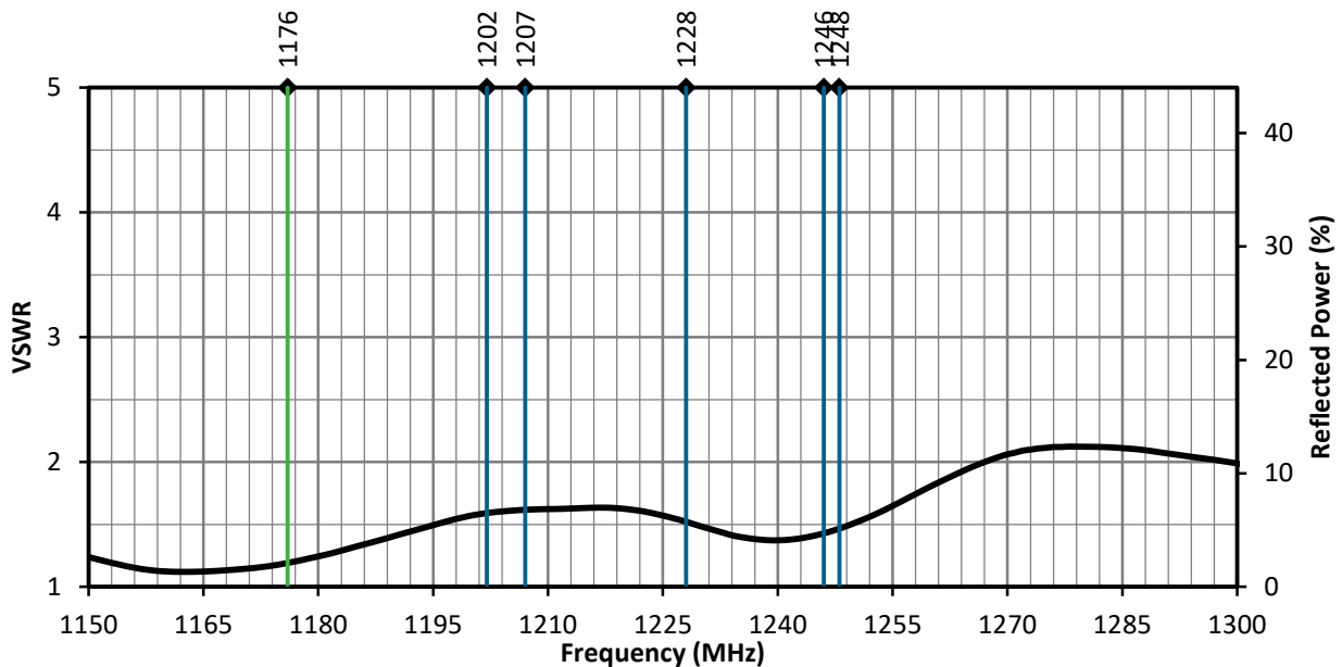
Figure 4. ANT-GCRM-L125A VSWR, L2 and L5 Bands
