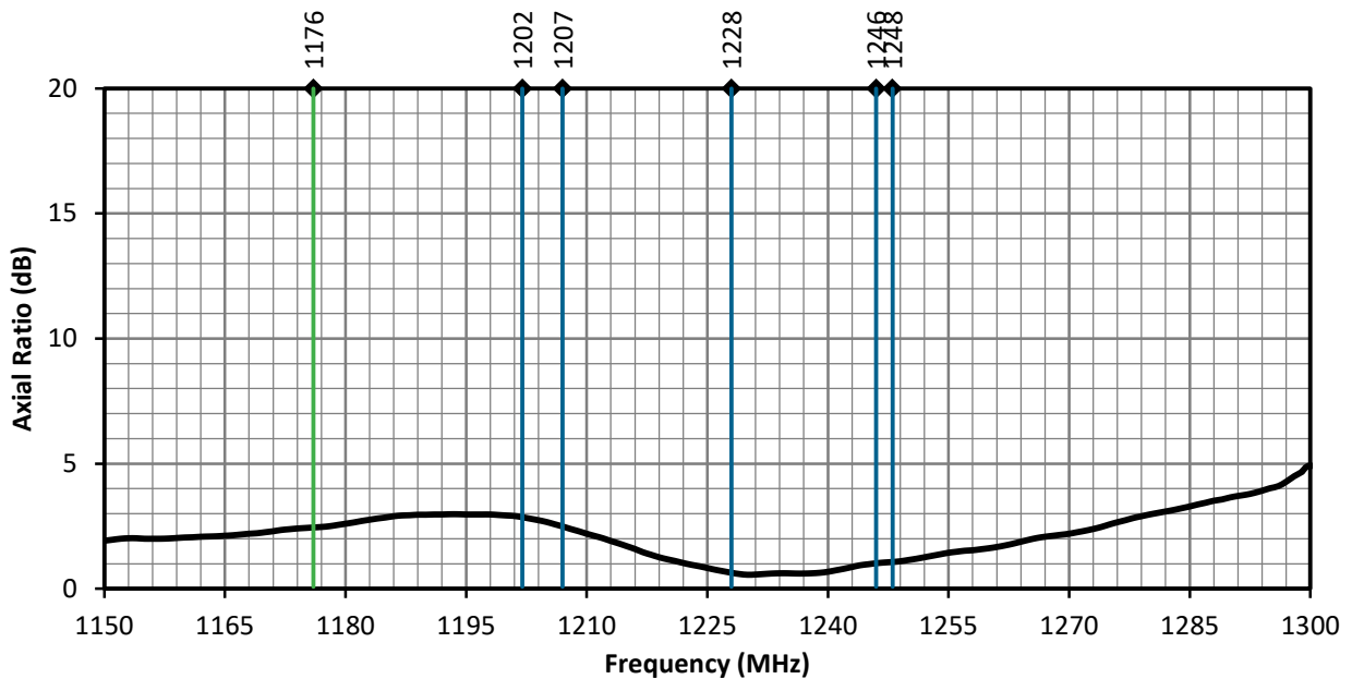
Figure 10. ANT-GCRM-L125A Antenna Axial Ratio, L2 and L5 Bands
