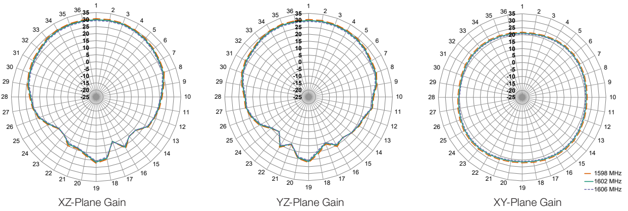
Figure 11. ANT-GCRM-L125A Radiation Patterns
