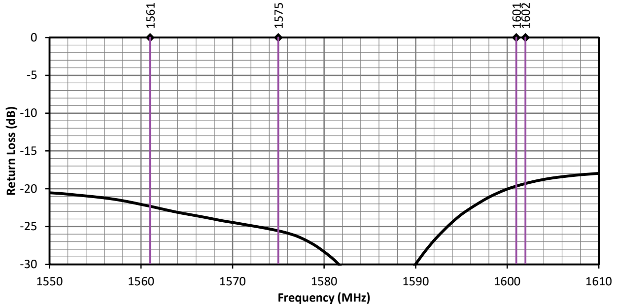
Figure 5. ANT-GCRM-L125A Return Loss, L1 Band
