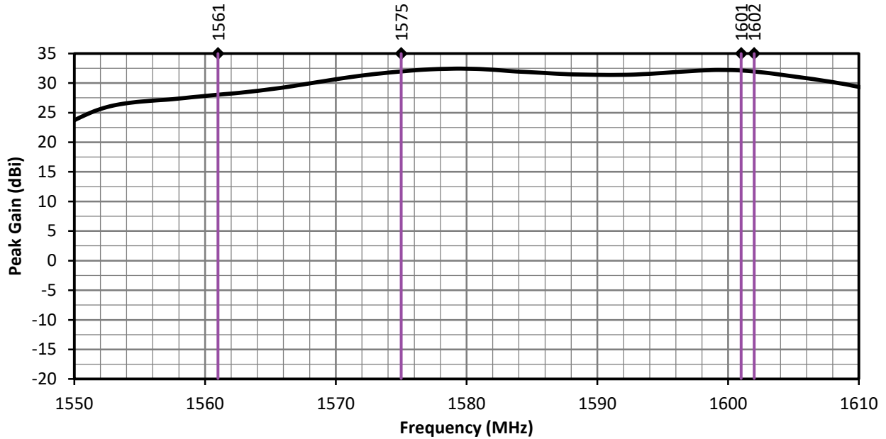
Figure 7. ANT-GNRM-L12A Series Antenna Peak Gain, L1 Band
