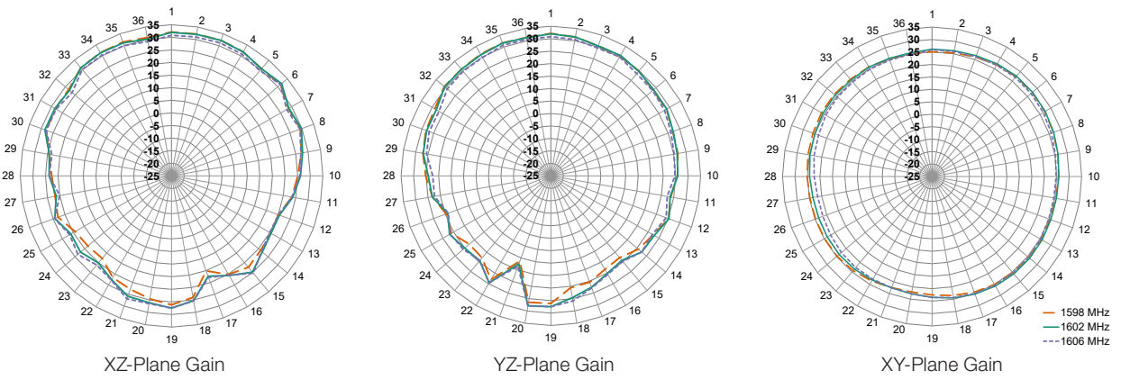
Figure 11. ANT-GCRM-L12A Radiation Patterns
