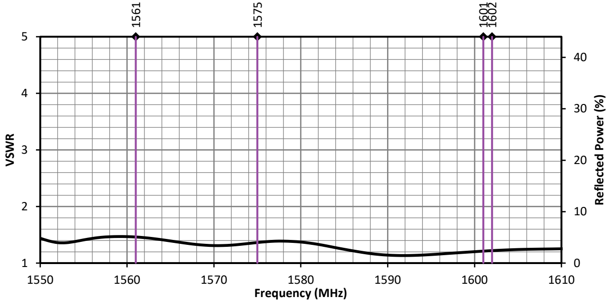
Figure 3. ANT-GNRM-L12A Series Antenna VSWR, L1 Band
