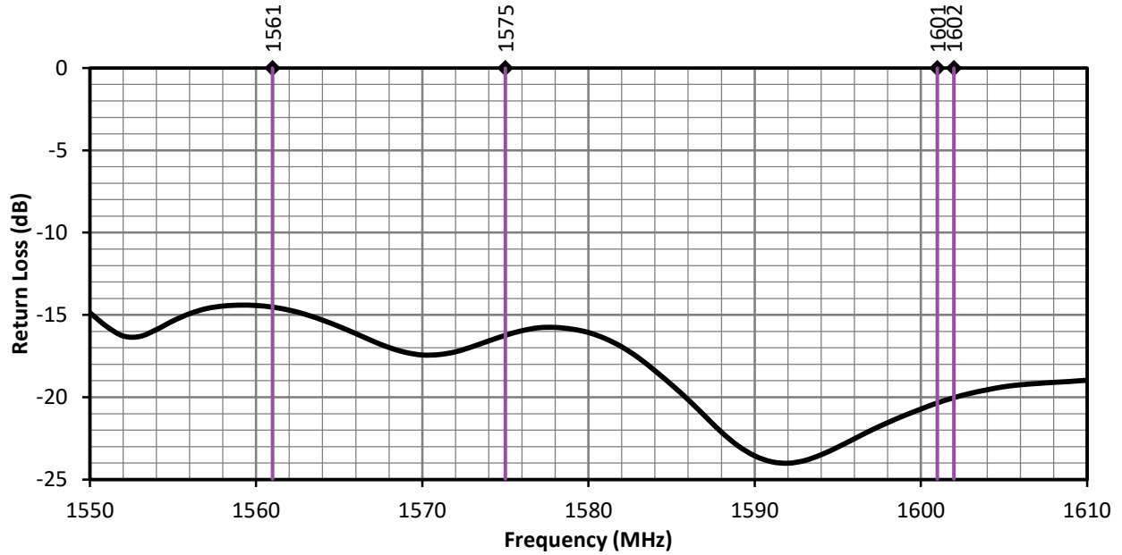
Figure 5. ANT-GCRM-L12A Series Antenna Return Loss, L1 Band
