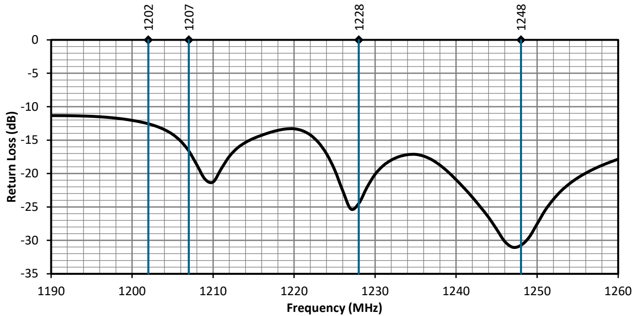
Figure 6. ANT-GCRM-L12A Series Antenna Return Loss, L2 Band
