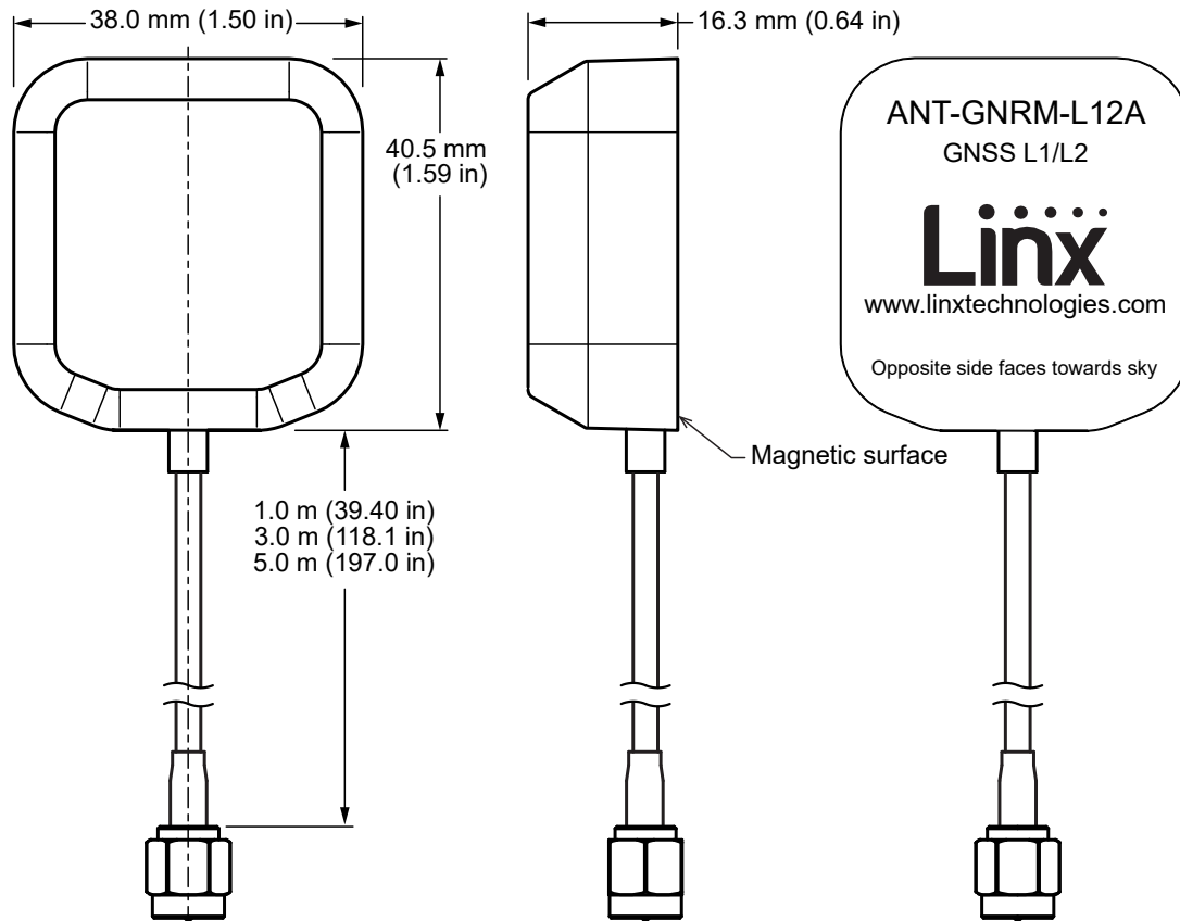
Figure 1. ANT-GCRM-L12A Series Antenna Dimensions
