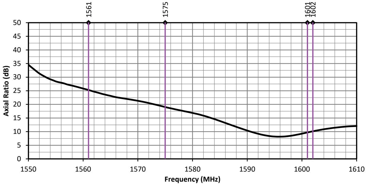
Figure 9. ANT-GCRM-L12A Series Antenna Axial Ratio, L1 Band
