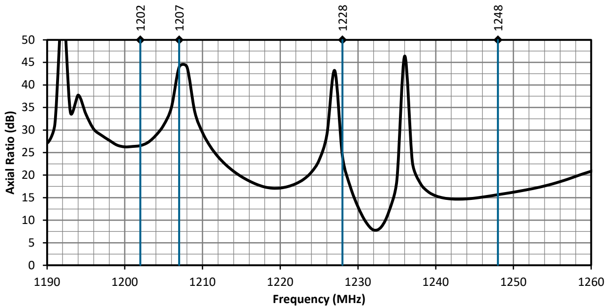
Figure 10. ANT-GCRM-L12A Series Antenna Axial Ratio, L2 Band
