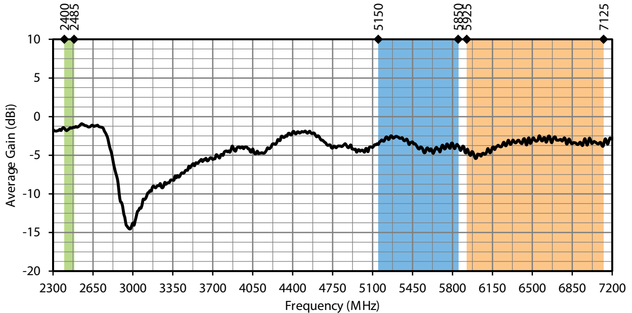
Figure 14. W63WS1 Antenna Average Gain, Edge-Bent
