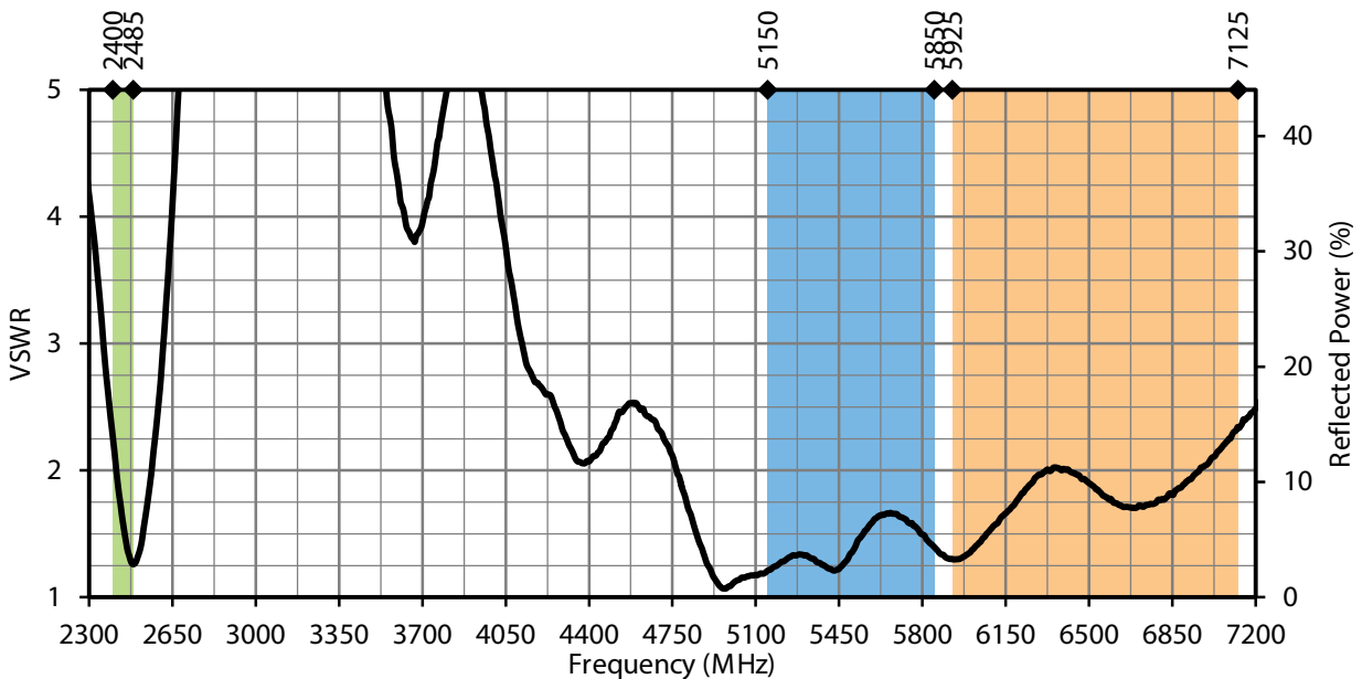
Figure 4. W63WS1 VSWR, Straight
