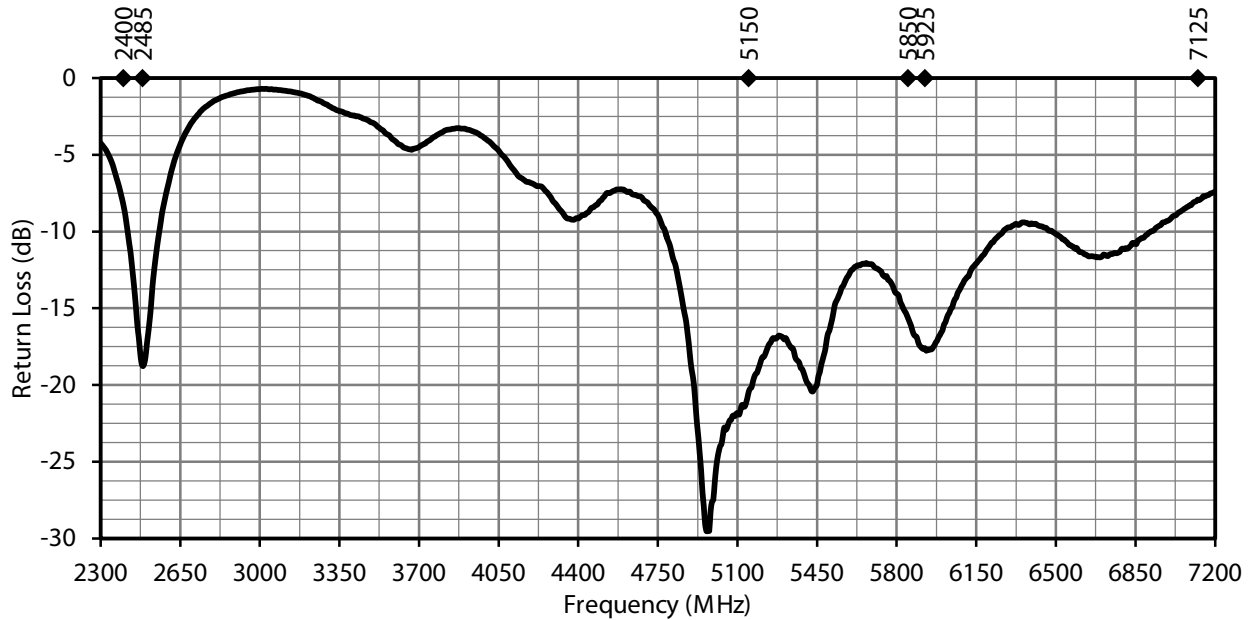
Figure 5. W63WS1 Return Loss, Straight
