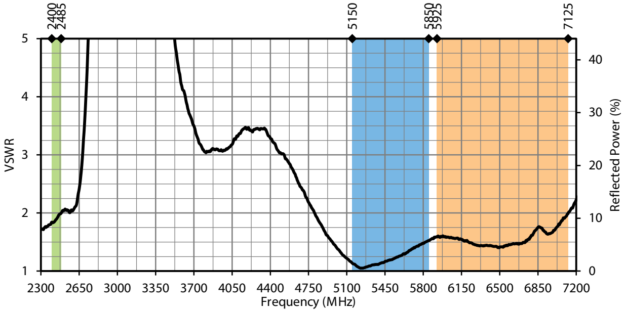
Figure 11. W63WS1 Antenna VSWR, Edge-Bent
