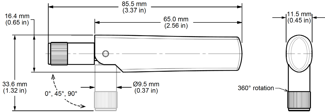
Figure 1. ANT-W63WS1 Antenna Product Dimensions
