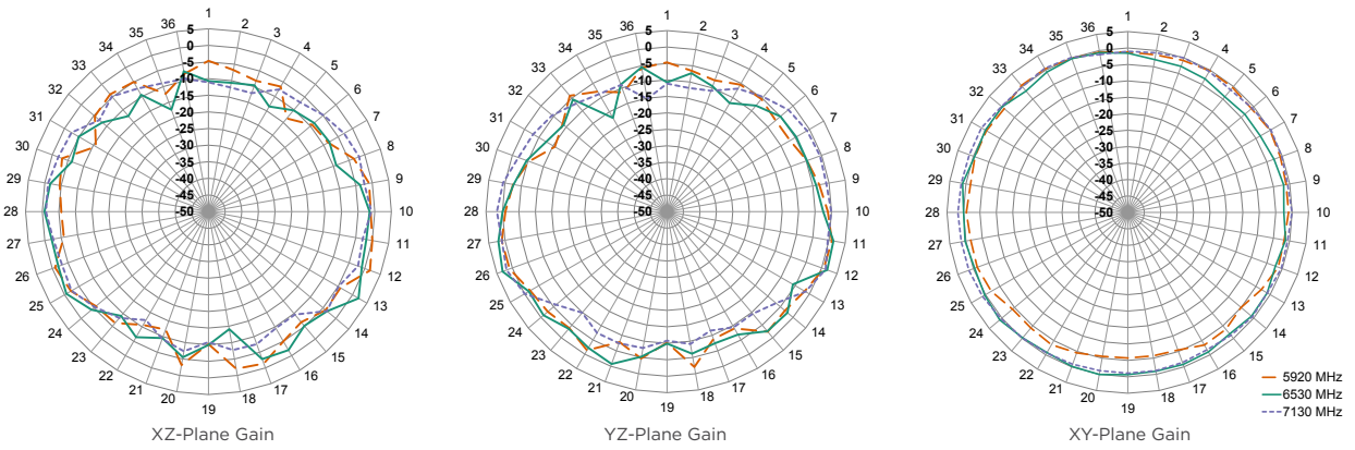
Figure 9. ANT-W63WS1 Antenna Radiation Patterns, Straight
