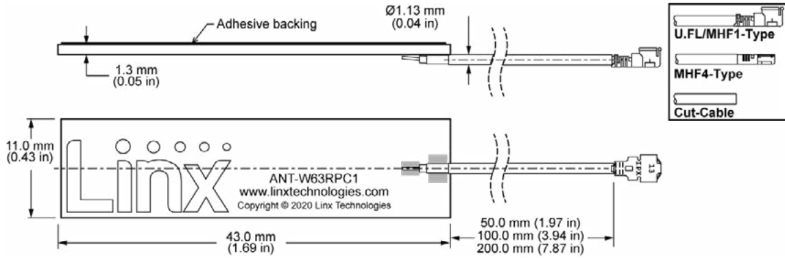
Figure 1. W63RPC1 Series Product Dimensions
