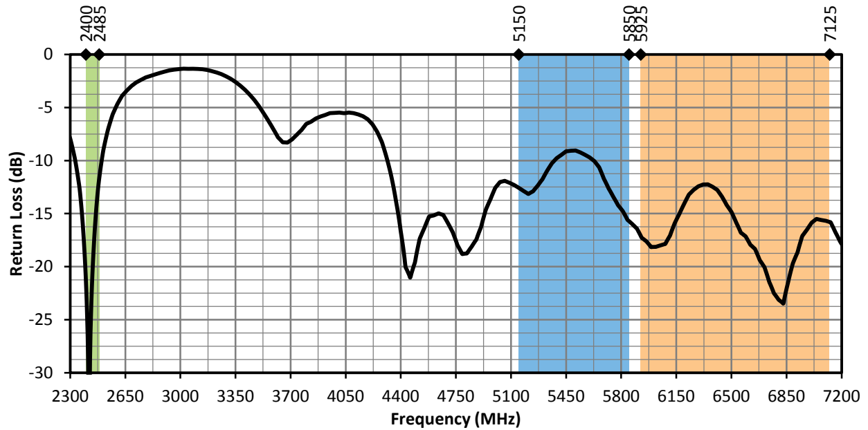
Figure 3. W63RPC1 Return Loss with Frequency Band Highlights
