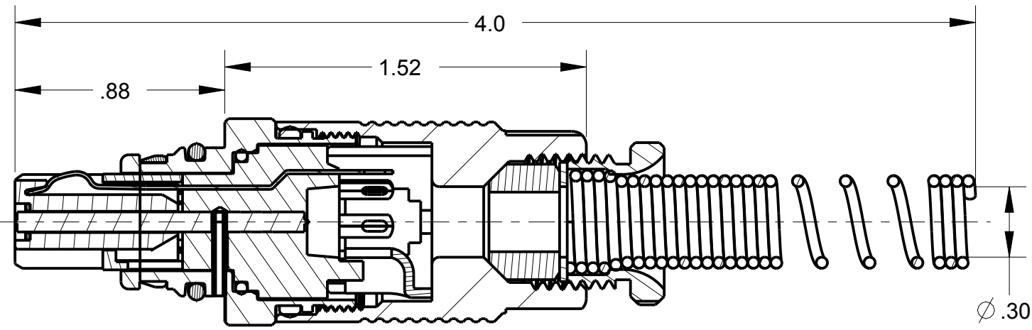
SECTION Z-Z
