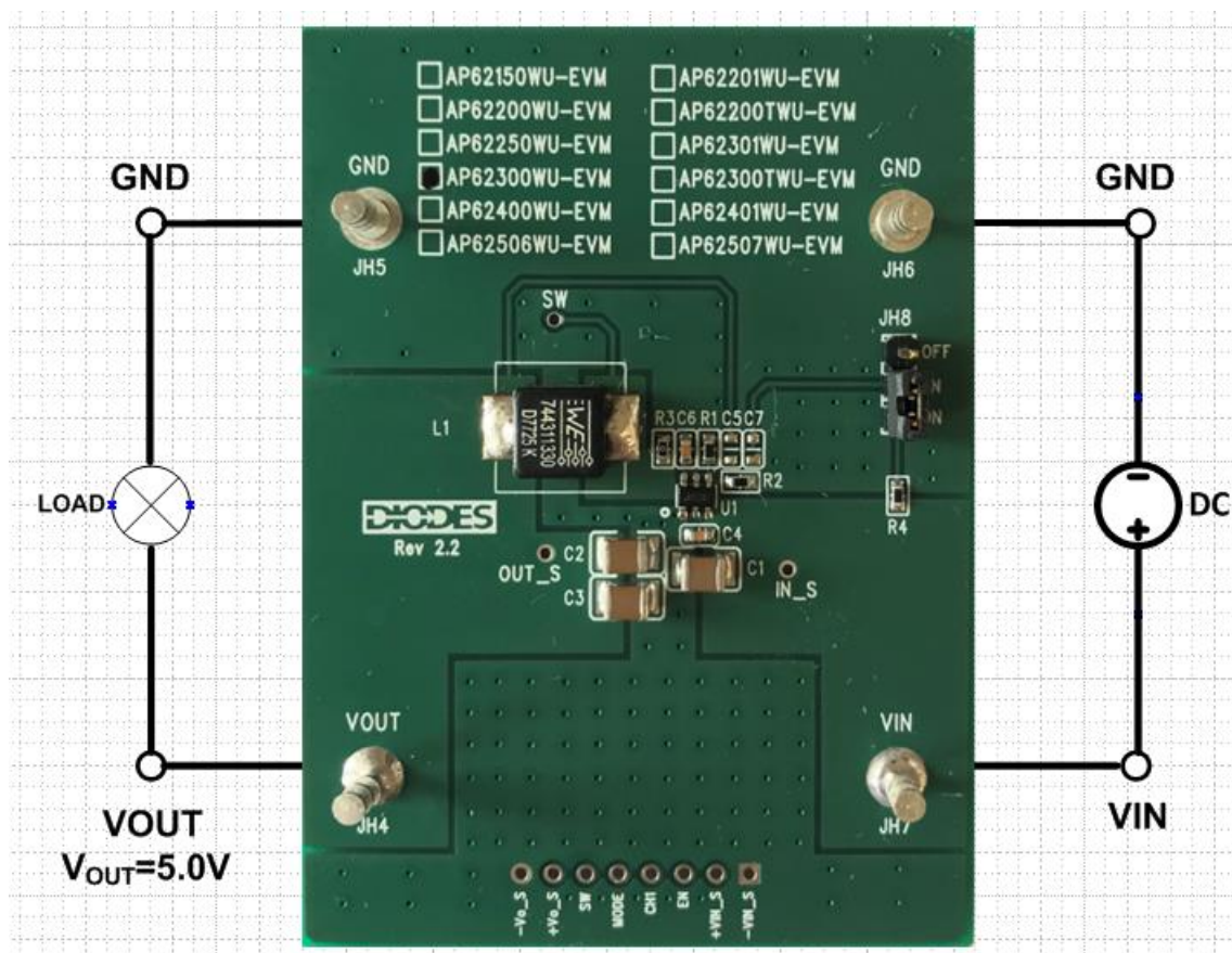
Figure 2. AP62300WU-EVM
