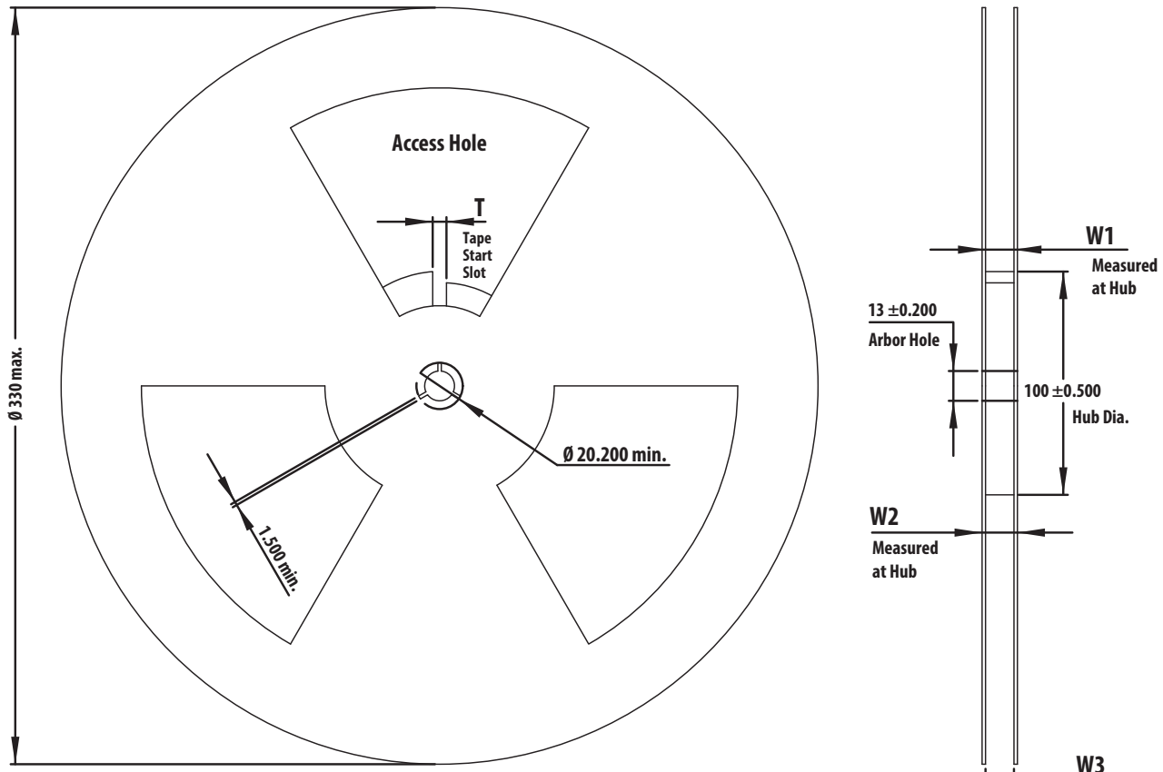
Figure 20 Reel Dimensions
