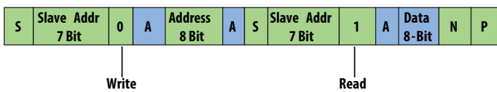
Figure 12 I 2 C Register Read
