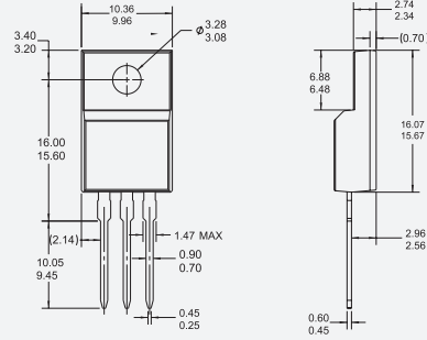
TO-220 [KF]
