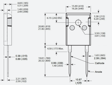
TO-247 2-Lead
