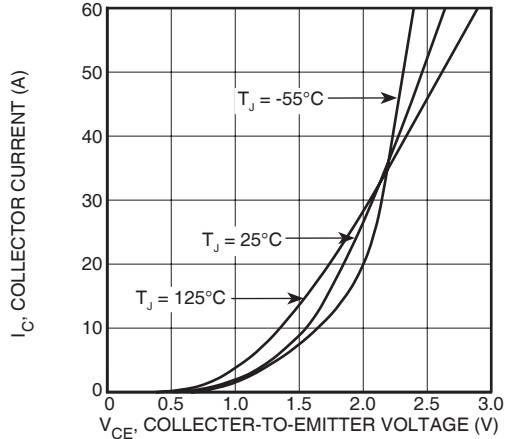
FIGURE 1, Output Characteristics(T J = 25°C)
