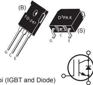
Combi (IGBT and Diode)
