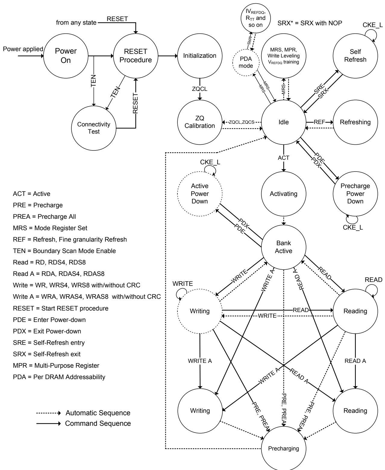
Figure 3. State Diagram
