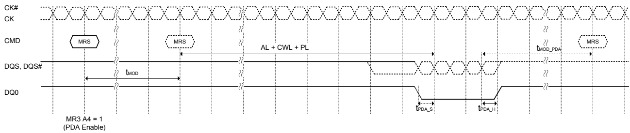
Figure 60. PDA using Burst Chop 4
