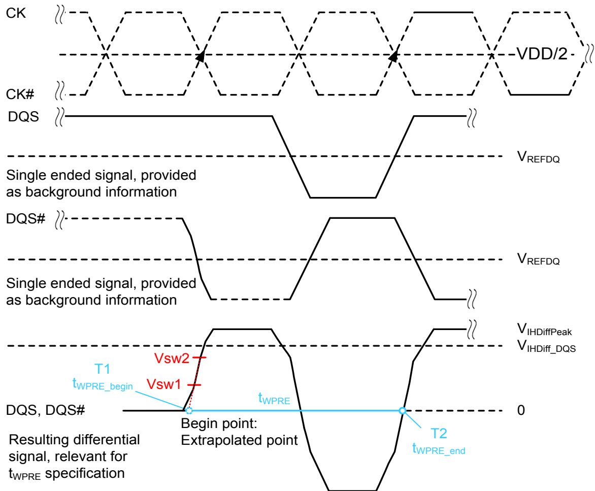
Figure 135. Method for calculating t WPRE transitions and endpoints
