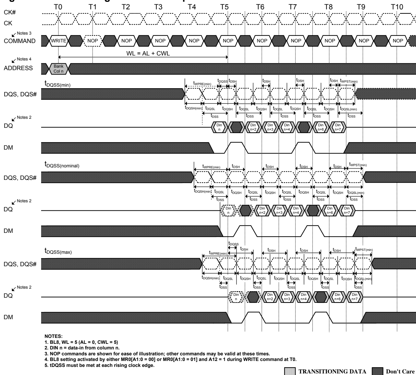
Figure 67. Write Timing Definition and parameters
