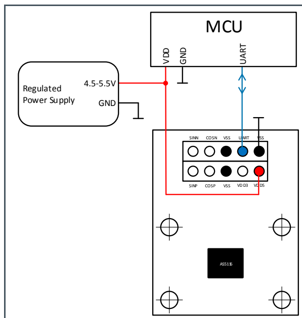
Figure 9: 5 V Operation
