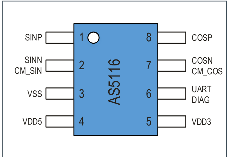
Figure 6: Sensor Pinout
