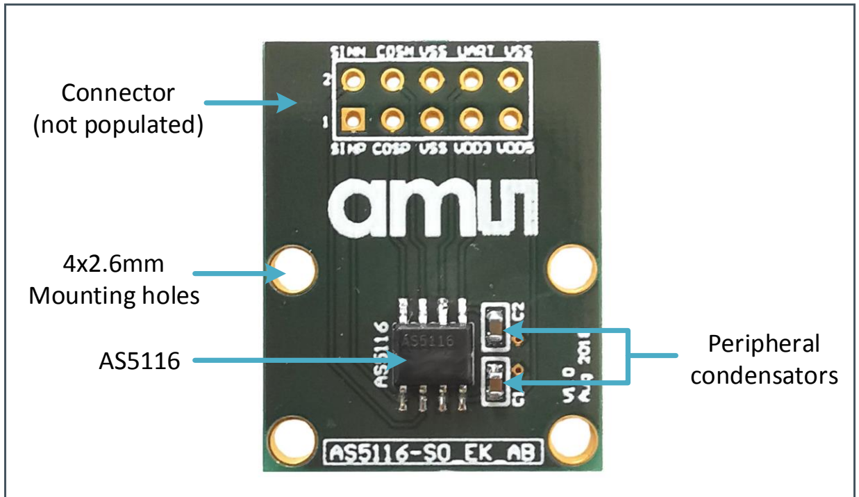
Figure 3: AS5116 Adapter Board
