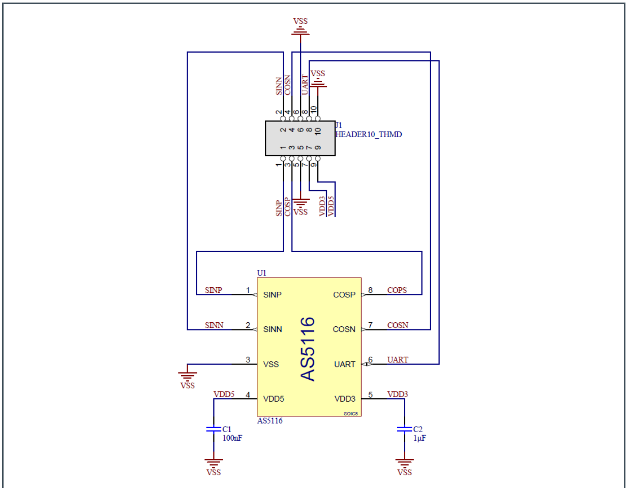
Figure 12: Schematic
