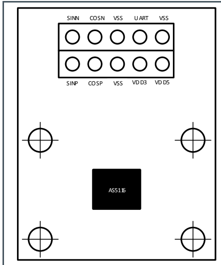
Figure 5: Adapter Board Pinout
