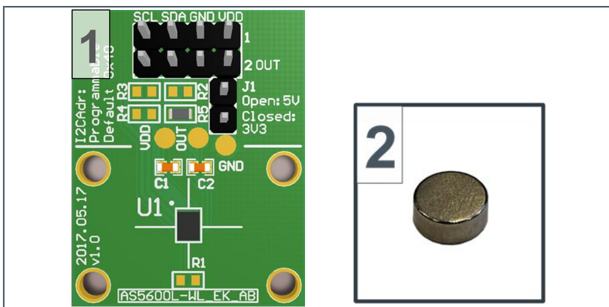
Figure 1: Kit Content
