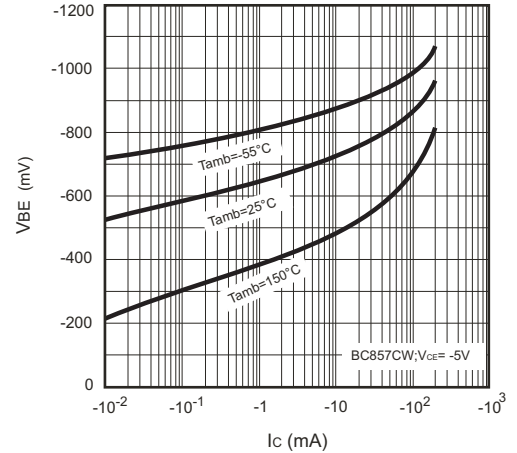
Fig.10- Base-Emitter Voltage as a function of collector current; typical values
